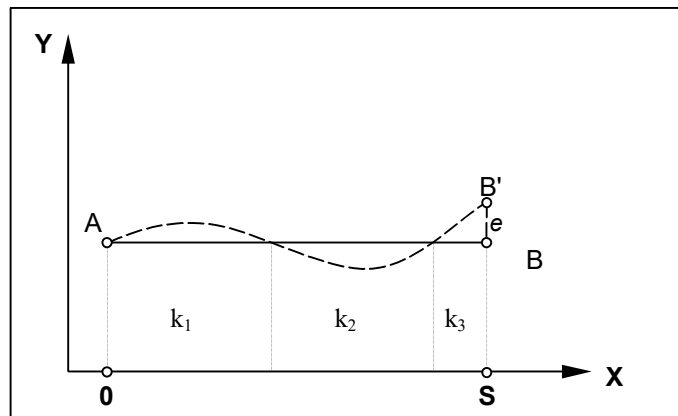
Figure 4-5. Effects of changeable gradients of temperature.
