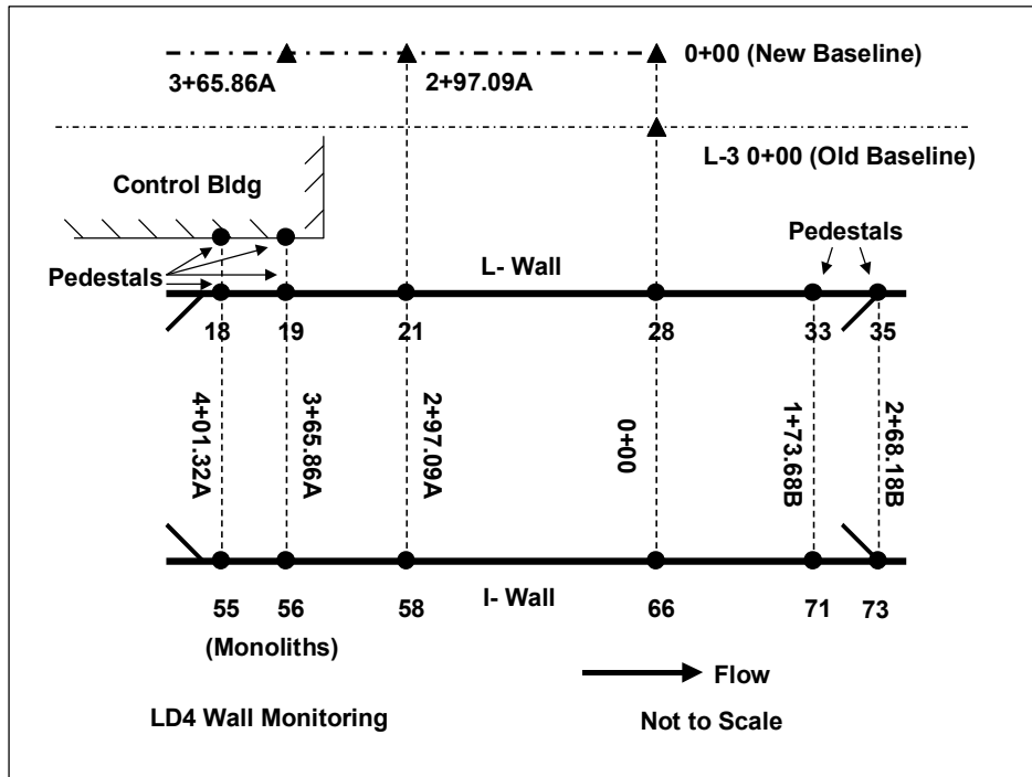
Figure B.3. Installation Plan and Measurement Scheme for conventional deformation surveys.
